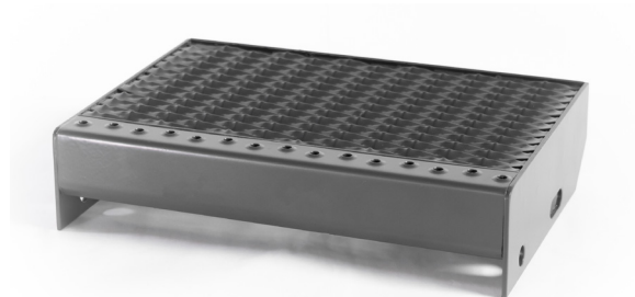
Tread with omnidirectional anti-slip expanded metal, Safe 45 × 13.4/5 mm
